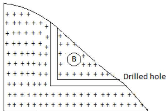
Figure 1.4 Quarrying by channelling
